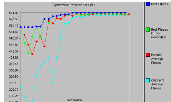
Figure 4: Optimization Run Graph
