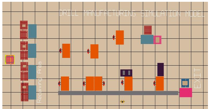
b) Top-View for New Layout Model
