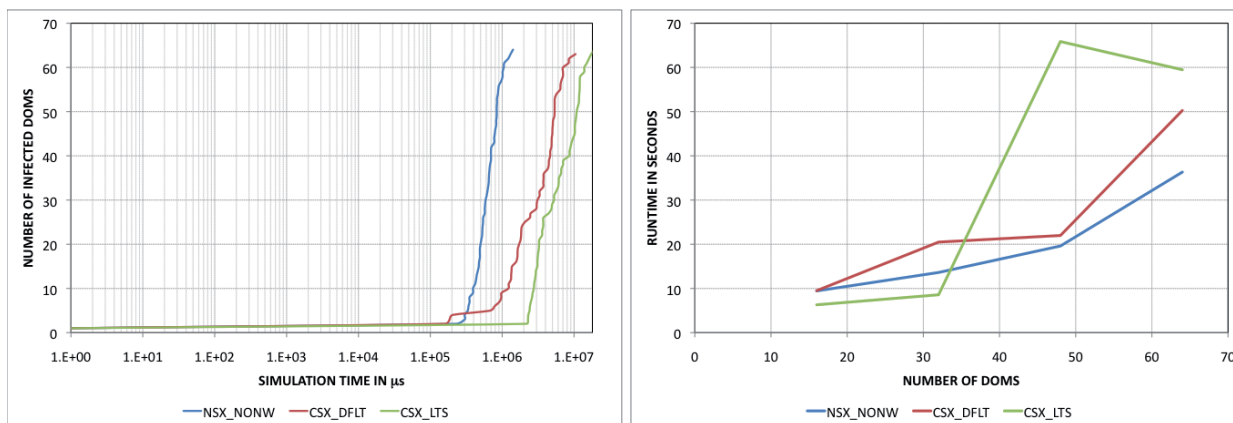
Figure 4: Infection propagation curve for 64-DOM (left) and runtime curves for 16, 32, 48 and 64 DOM scenarios (right) for cyber security benchmarks involving both CSX setups and, NSX without network control setup
