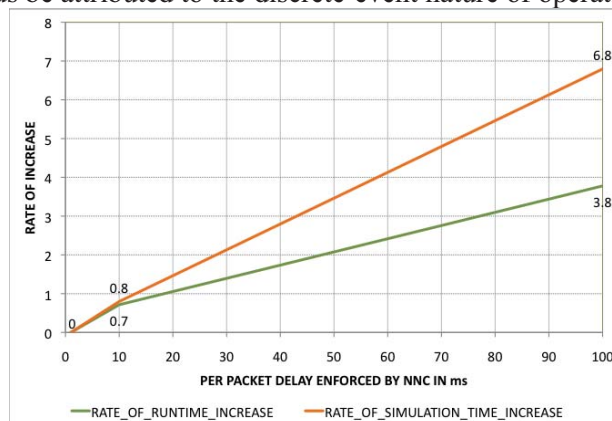
Figure 7: Rate of increase in the runtime and the simulation time with the increase in virtual packet delay
