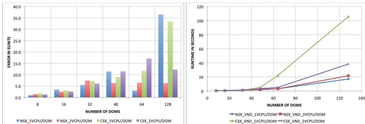
Figure 3: VND benchmark error plots (left); VND benchmark runtime plots (right)
