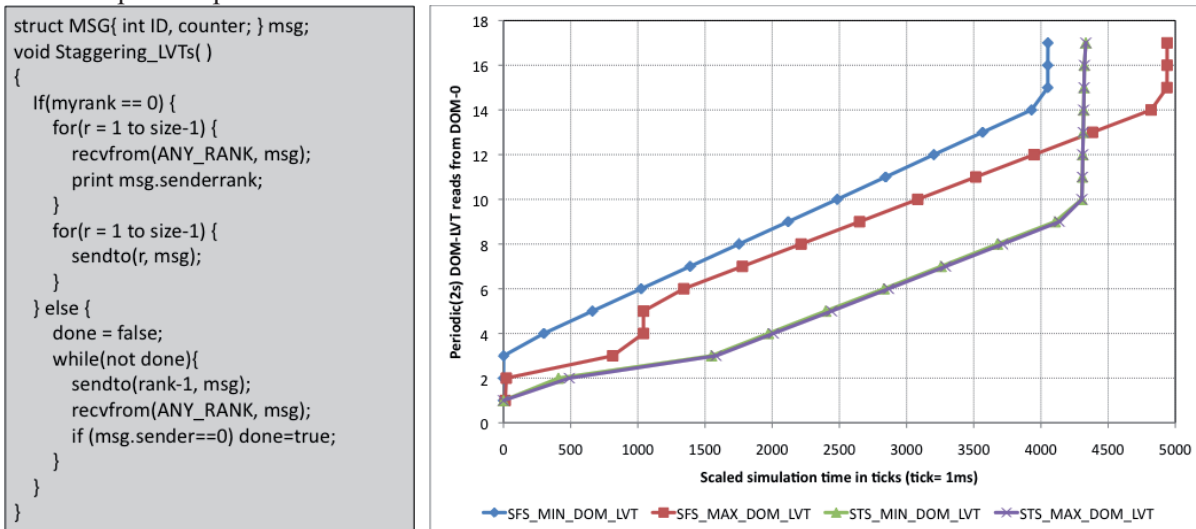
Figure 1: Algorithm to test staggering virtual timelines (left); Experiment results comparing simulation time divergence in SFS and STS (right).
