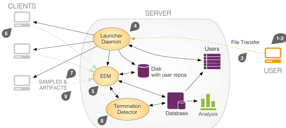
Figure 1: High level architecture of SAFE.
