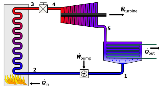
Figure 1: Rankine Cycle
