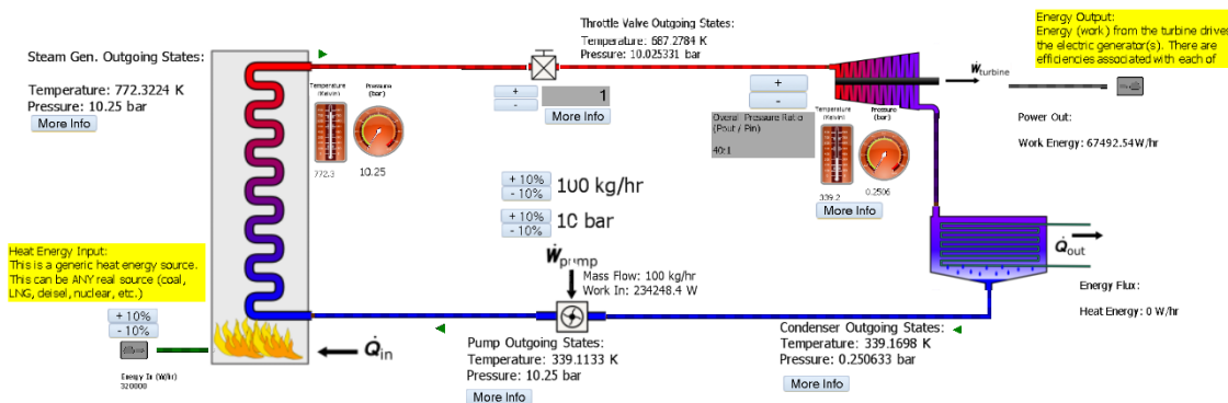
Figure 4: Running Rankine Cycle
