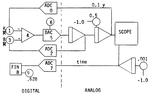
Figure 3. Second Derivative Calculation on Digital
