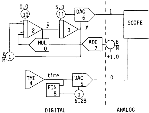
Figure 2. Parameter Change With Analog Pot
