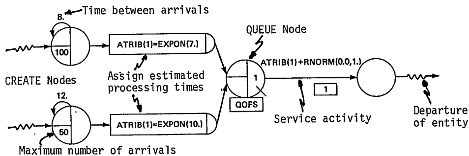
Figure 1. Network Model of a Multiple Entity, Single Server Queuing Situation
