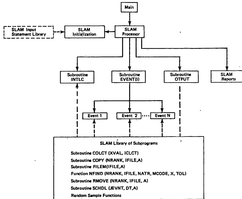
Figure 2. SLAM Organization for Discrete Event Modeling
