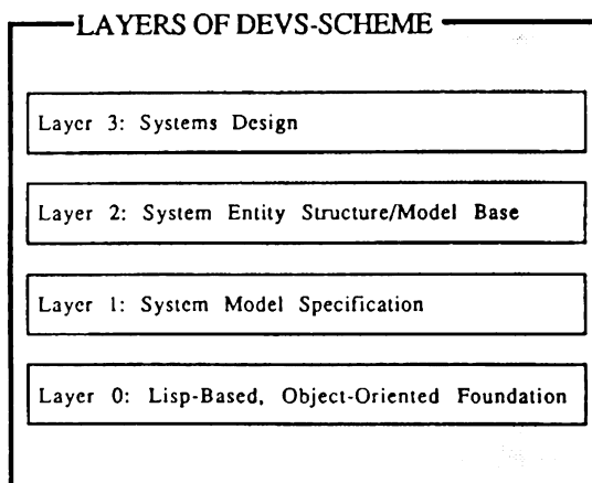
Figure1 Layers of DEVS-Scheme
