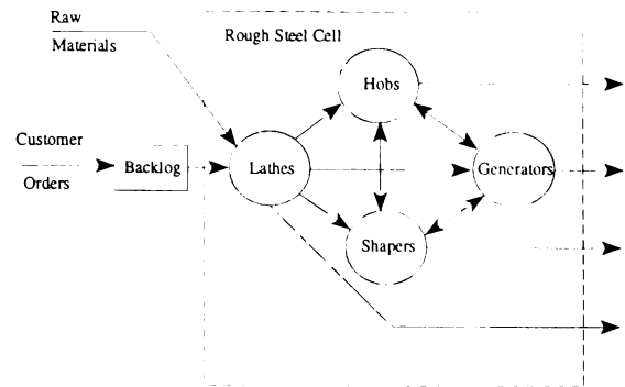
Figure 4: System Studied
