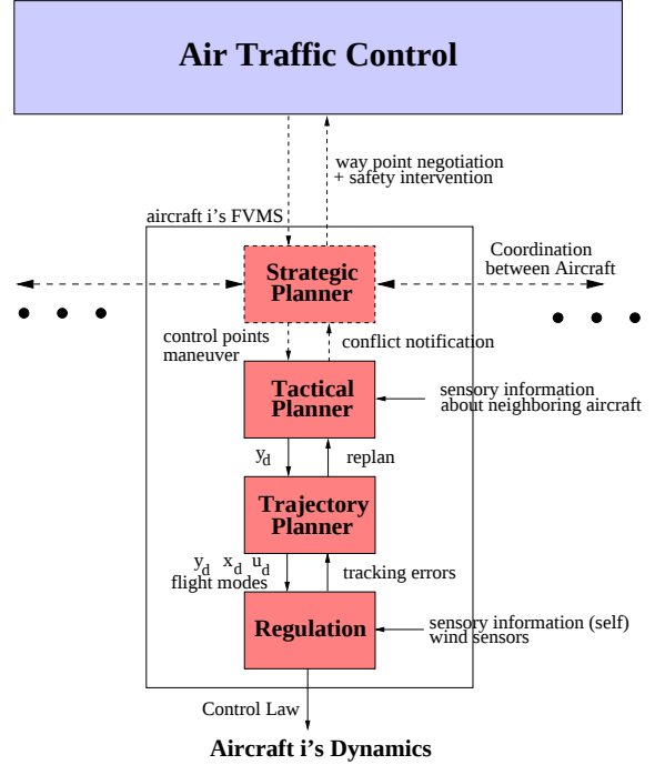
Figure 1: Proposed FVMS Architecture
