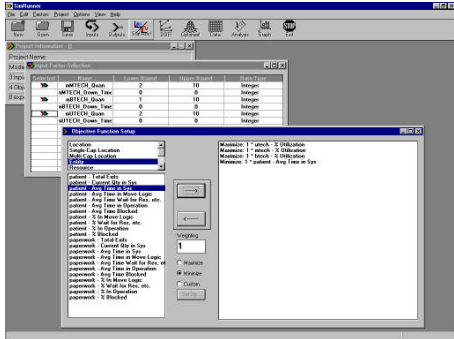
Figure 8: SimRunner Output Factors
