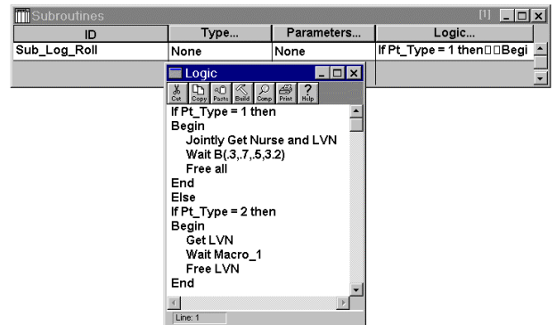
Figure 5: Subroutine and Macro Usage
