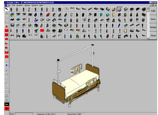
Figure 7: Graphic Editor
