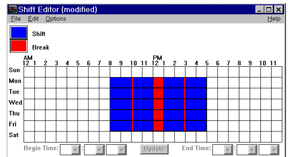
Figure 6: Shift Editor
