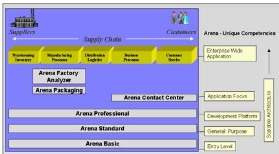
Figure 1: Arena Software Architecture
