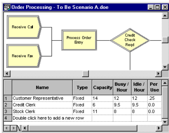
Figure 2: Arena Basic Edition Flowchart and Data
