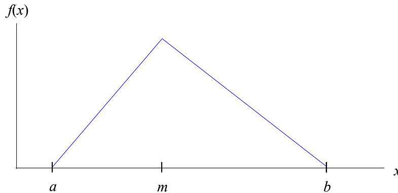
Figure 8: Triangular density function on the interval [a, b] with mode m
