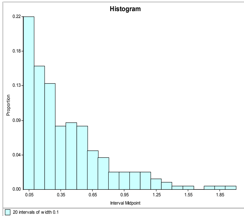
Figure 3: Histogram of 219 interarrival times to a drive-up bank
