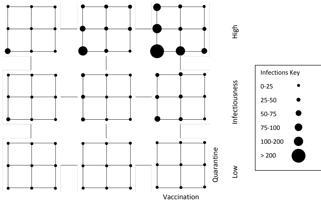
Figure 7: Infections Key Low Days Contagious High Vaccination Influenza study in Beeler, Aleman and Carter (2012)
