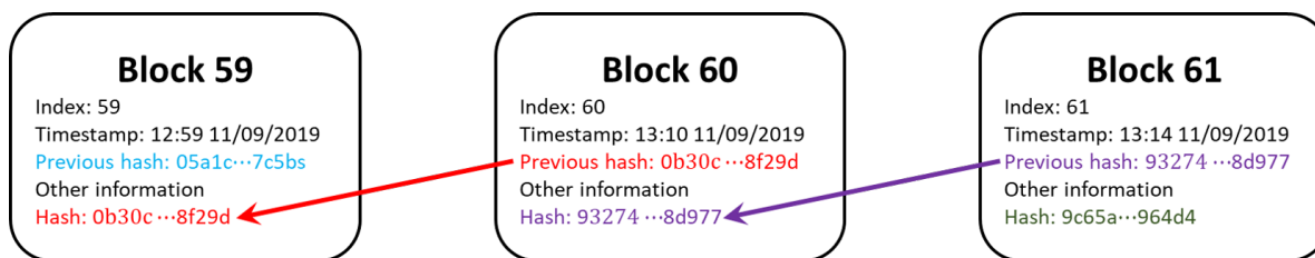
Figure 1: Blockchain demonstration.
