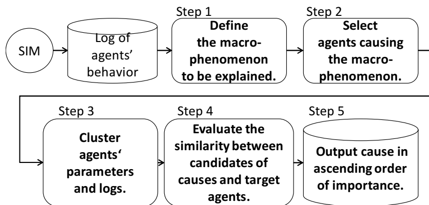
Figure 2: Conventional micro-dynamics method.
