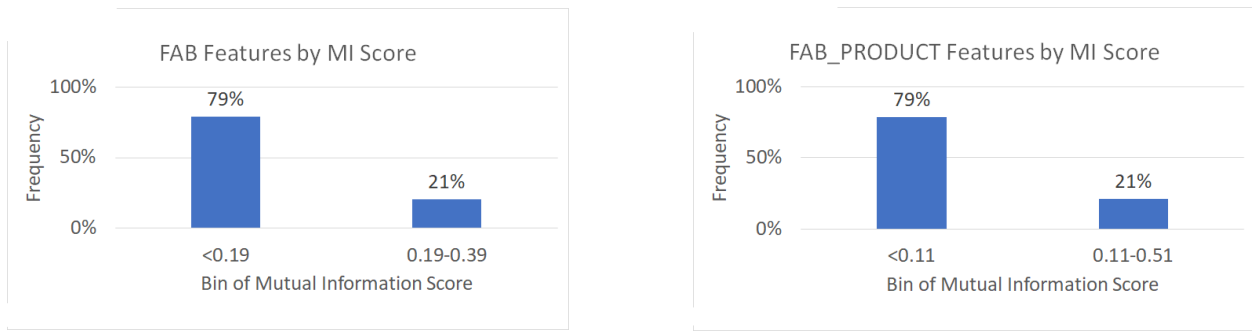
Figure 2: Frequency diagram of FAB and FAB_PRODUCT features by mutual information score.
