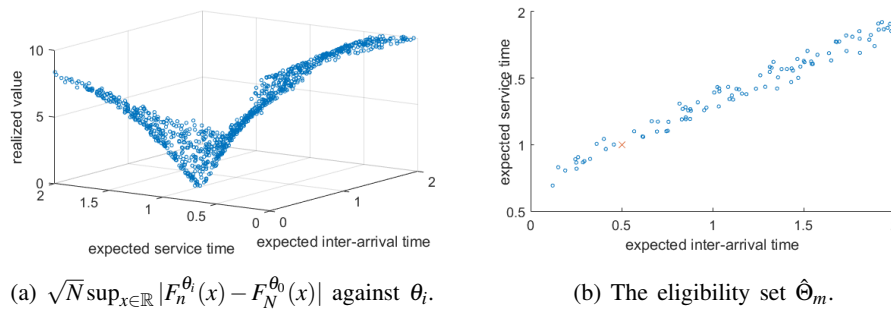
Figure 2: Apply Algorithm 1 to calibrate (\lambda, \mu) .
