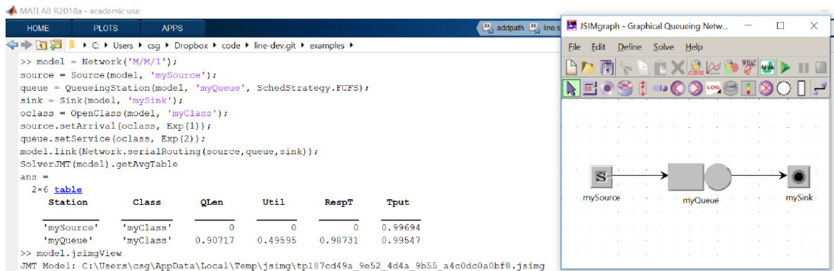
Figure 1: M/M/1 simulation in LINE and visualization via export to JMT
