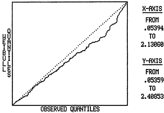
Figure 4: An Example Q-Q Plot Using A Weibull Distribution
