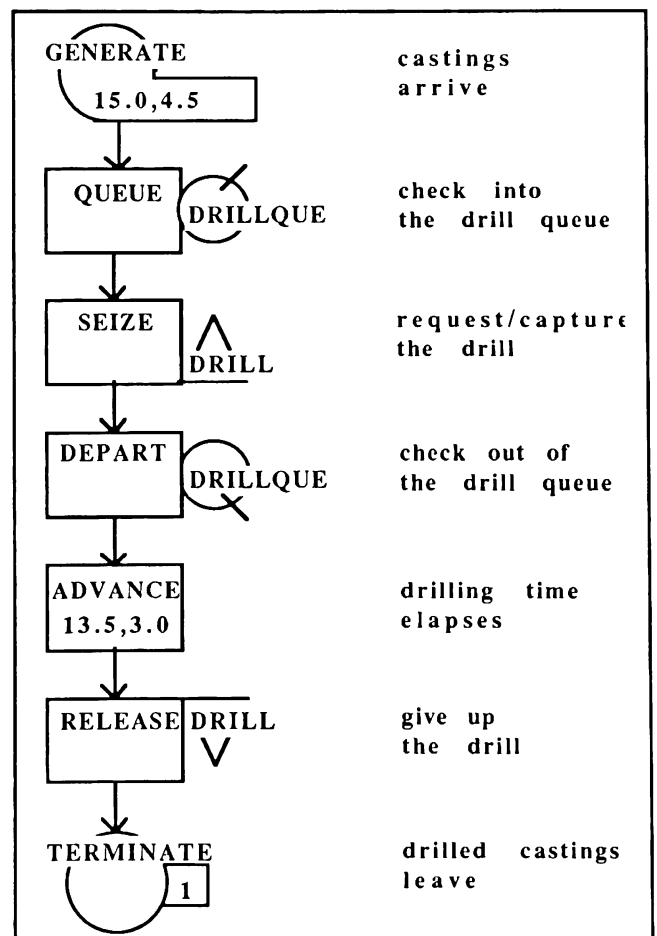
Figure A-1: GPSS Block Diagram for a One-Line, One-Server Queuing System
